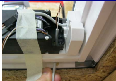
Wire routing for "C" sizes
